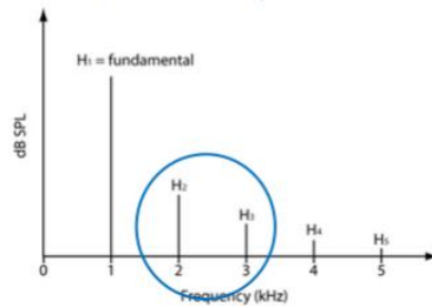
After THD Compensation
