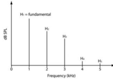
Before THD Compensation
